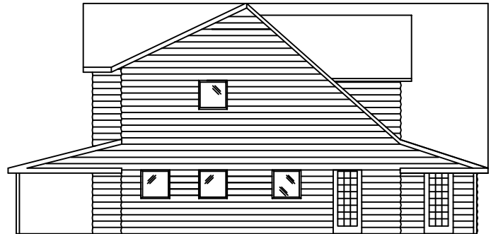
4 LEFT SIDE ELEVATION PLAN# 2L-44-02409-A 48'-0"
